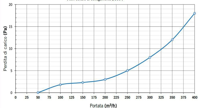
box SMART Large a 8 collarini Grey Ø75 posteriori (assiali)
